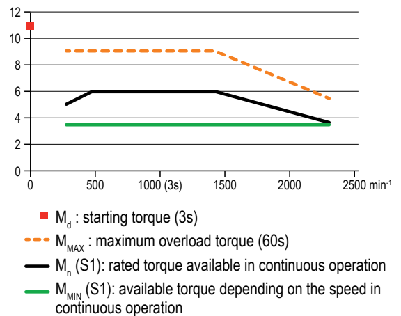
Orthobloc 0.25 to 7.5 kW up to 23,500 Nm
