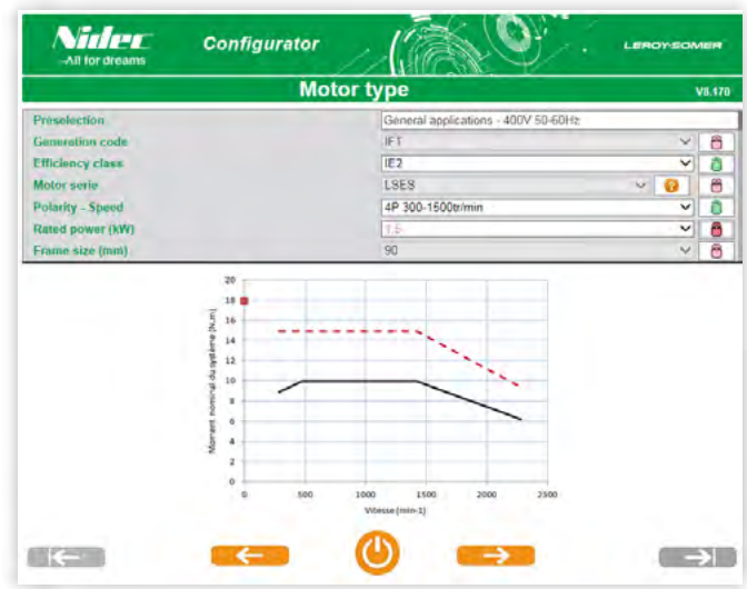
Drive & motor selection
