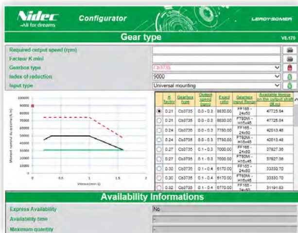
Gearbox selection, linked to motor selection
